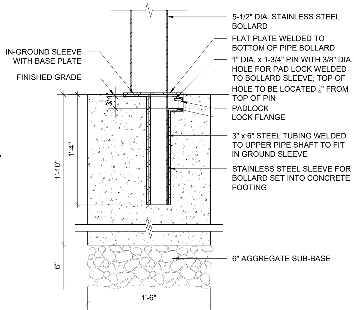
STAINLESS STEEL BOLLARD - REMOVABLE: SECTION - B
