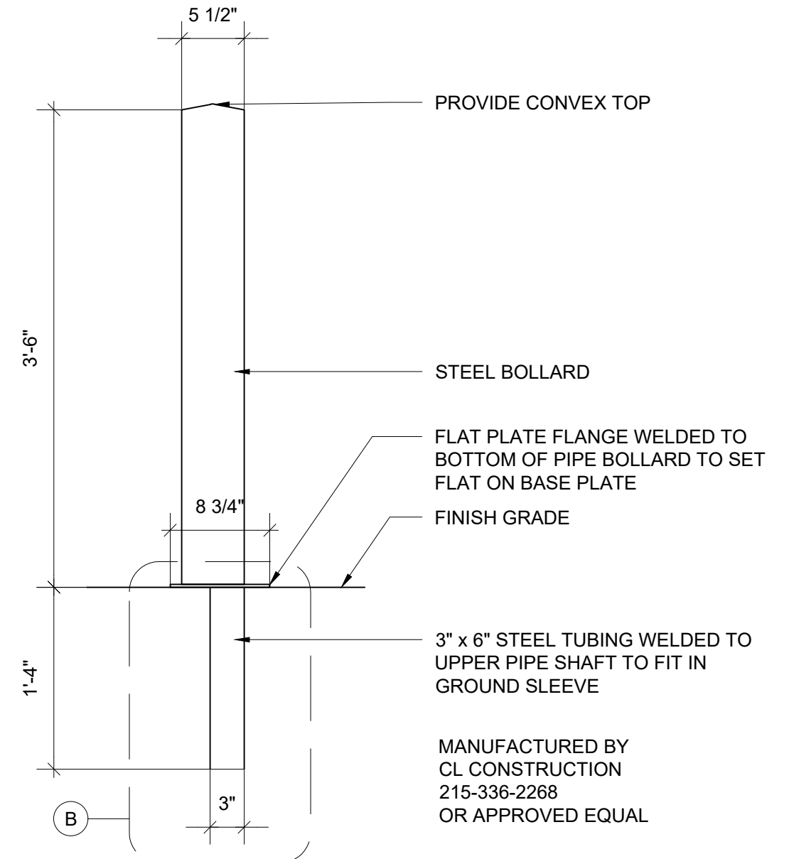
STAINLESS STEEL BOLLARD - REMOVABLE: SECTION - A
