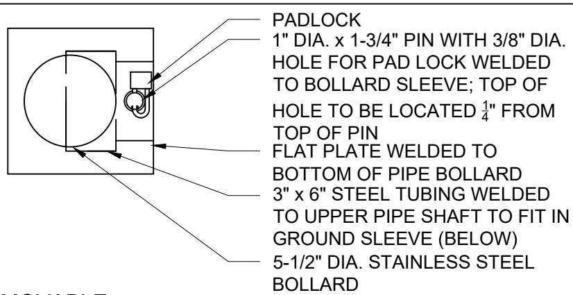
BOLLARD - REMOVABLE: PLAN
