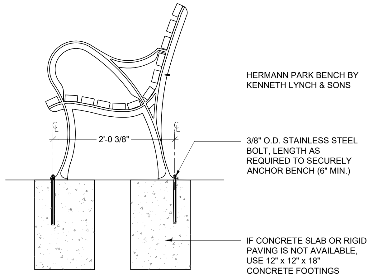
BENCH: SECTION
