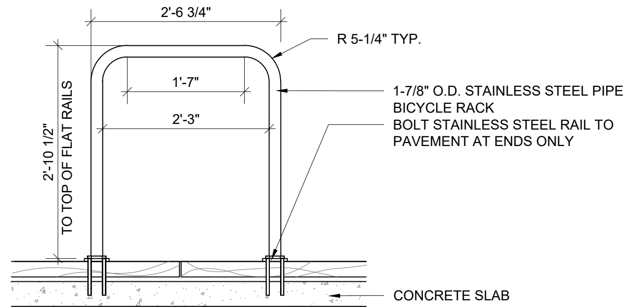
BICYCLE RACKS ON RAILS: SECTION
