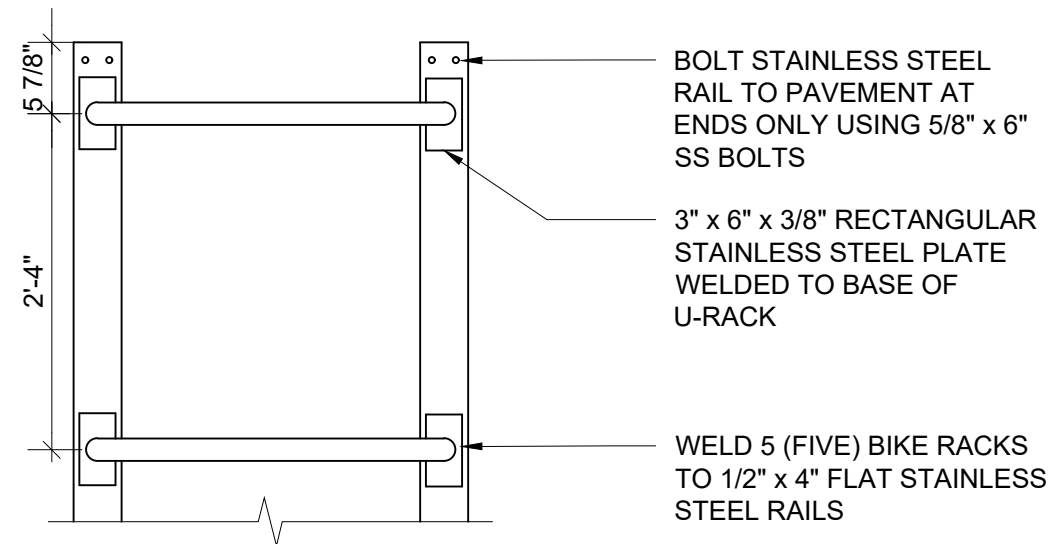
BICYCLE RACKS ON RAILS: PLAN
