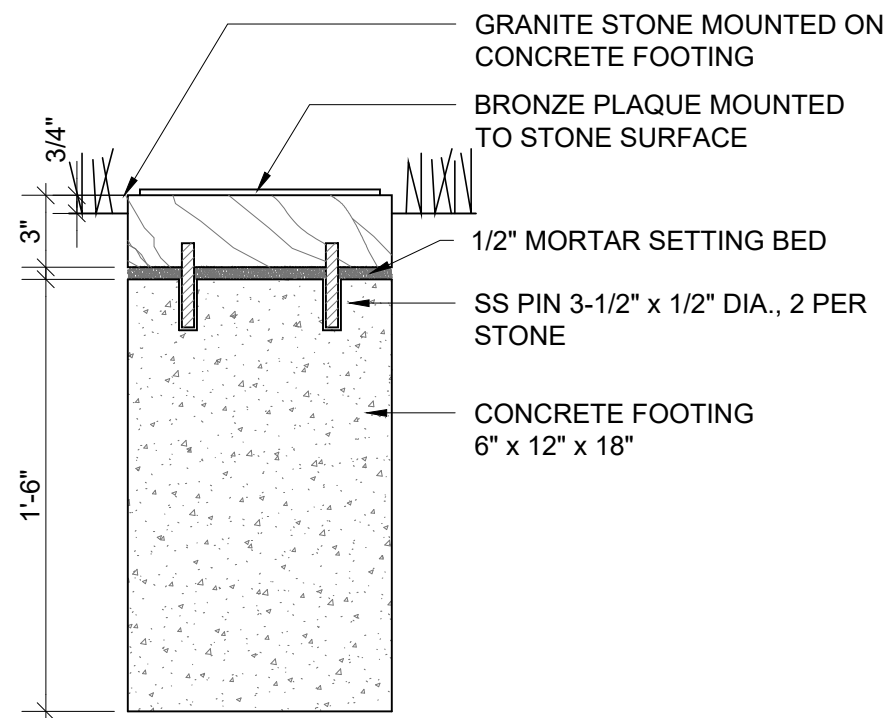
SCULPTURE PLAQUE: SECTION
