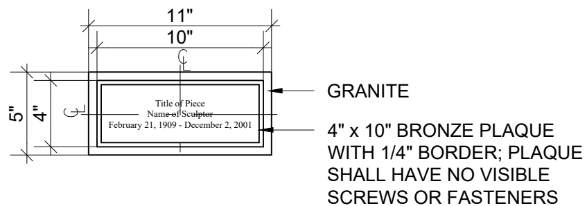
SCULPTURE PLAQUE: PLAN
