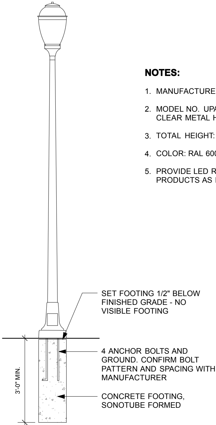
PEDESTRIAN POLE-MOUNTED LIGHT: SECTION SCALE: 1/2"=1'-0"
