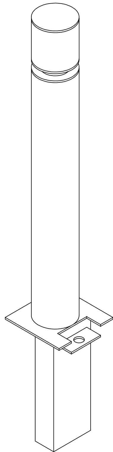
PAINTED BOLLARD - REMOVABLE: ISOMETRIC
