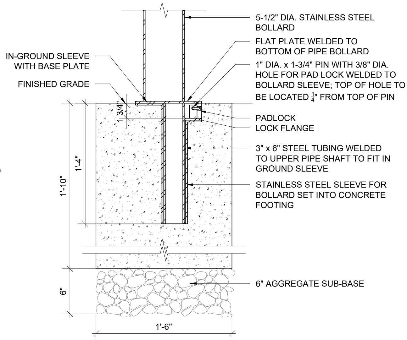
PAINTED BOLLARD - REMOVABLE: SECTION - B
