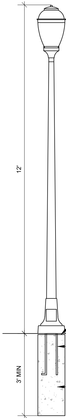
PEDESTRIAN POLE-MOUNTED LIGHT: SECTION SCALE: 1/2"=1'-0"
